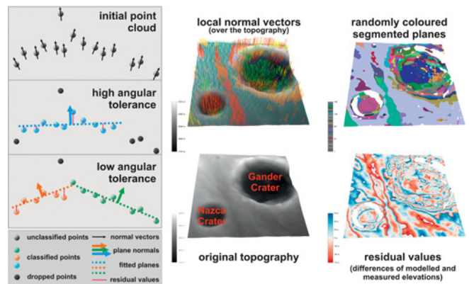
Principle of segmentation algorithm (left) and sequence of processing steps (right, clockwise from original topography).
