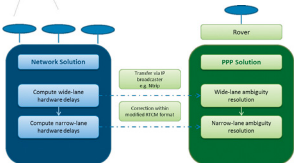
Uncalibrated Hardware Delays (UHD) broadcasting scheme. © PPP-Serve
