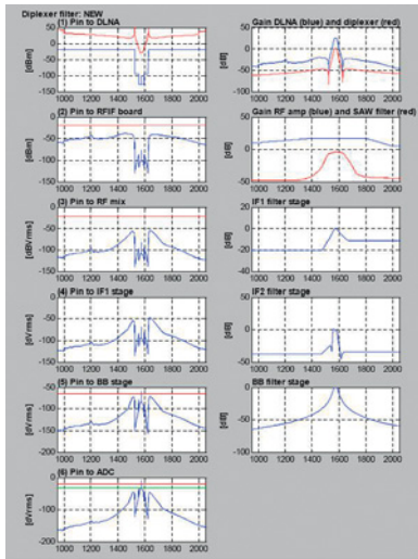
Example of RUAG's RFC analysis tool showing the L1 band. © RUAG Space GmbH
