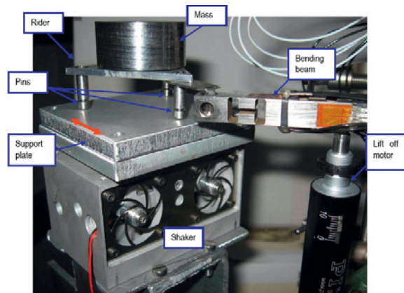
First prototype (shaker and measuring unit) mounted in vacuum chamber for first tests.
