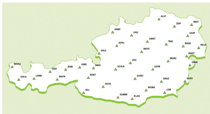
EPOSA GNSS station network. © PPP-Serve
