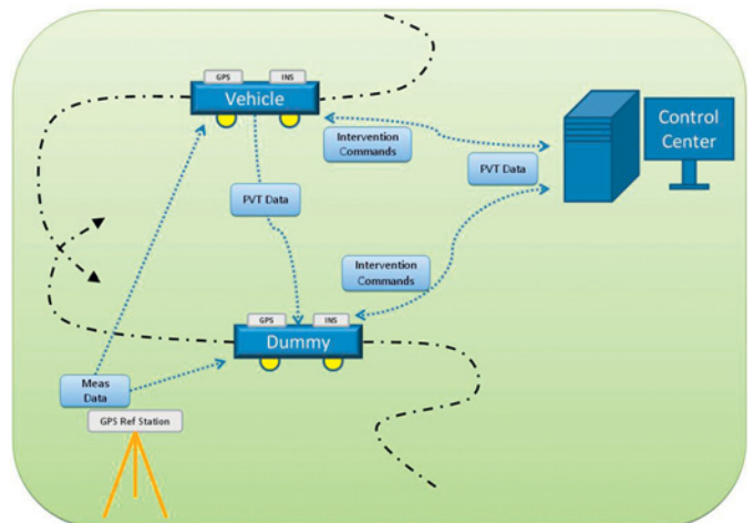
CrashPos system design. © Institute of Navigation, Graz University of Technology
