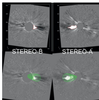
3D-POC results: CME observed from STEREO-A and STEREO-B (CME fronts are outlined in red). The direction of propagation of the CME is derived using a model (green mesh).
