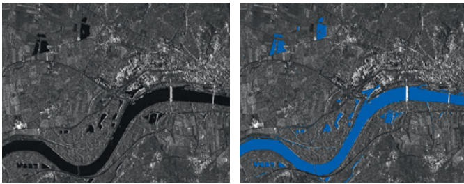
RAPIDEM prototype results of near real-time TerraSAR-X based water body detection. © GeoVille
