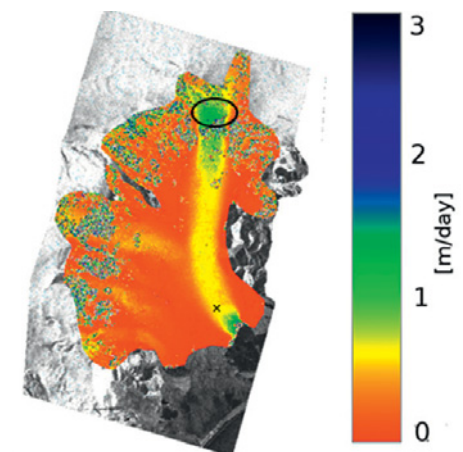
Surface displacement of Breiðamerkurjökull, Iceland, from COSMO-SkyMed data, acquired on 22 and 30 November 2010, overlaid on amplitude image. © ENVEO
