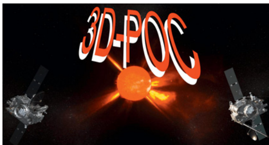
Artist's concept: STEREO-A and STEREO-B spacecraft observe the Sun from two vantage points to reveal 3D properties of dynamic eruptions. © NASA, adapted
