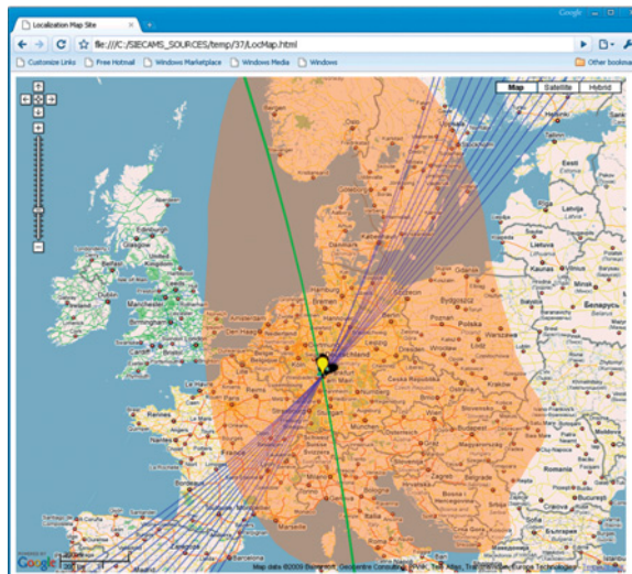
SIECAMS ILS continuous measurement. © Siemens 2012
