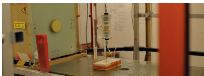
Calibration of the CDSM sensor in the Braunbek coil facility of TU Braunschweig, Germany. © ÖAW/IWF
