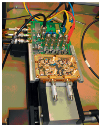
RFDC/G1 installed on test adaptor RF_ADAP. © RUAG Space GmbH
