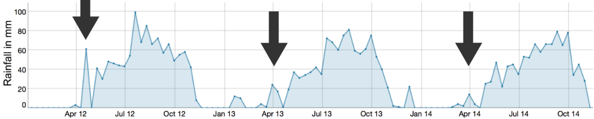
Satellite-based Rainfall (10-day accumulated Average) - Location (Lat/Lon): 19.25/8.00
